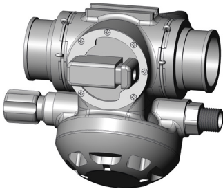
Bailout valve (BOV) with integrated Automatic diluent valve (ADV)
